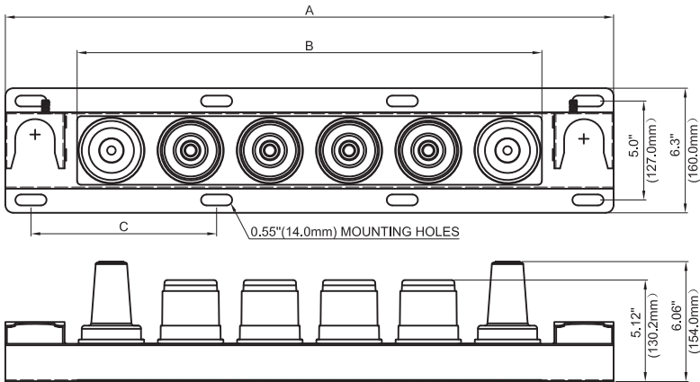
15/25 kV Model
