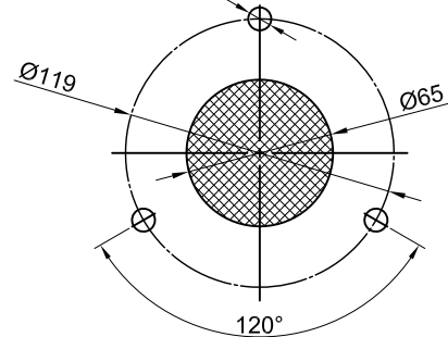
Figure 5: Recommended Tank Wall Dimensions
