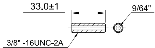
Figure 4: Removable Stud
