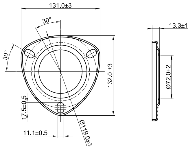
Figure 3: Stud Clamp with Flange (Zinc Dichromate Plate or Stainless Steel)
