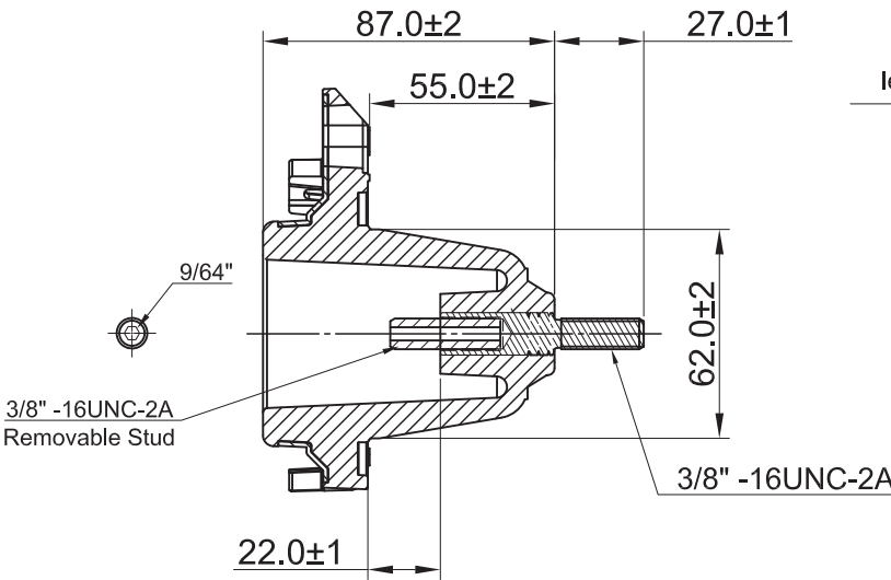
Fig. 3: 200A Bushing Well with Clamp & Removable Stud
