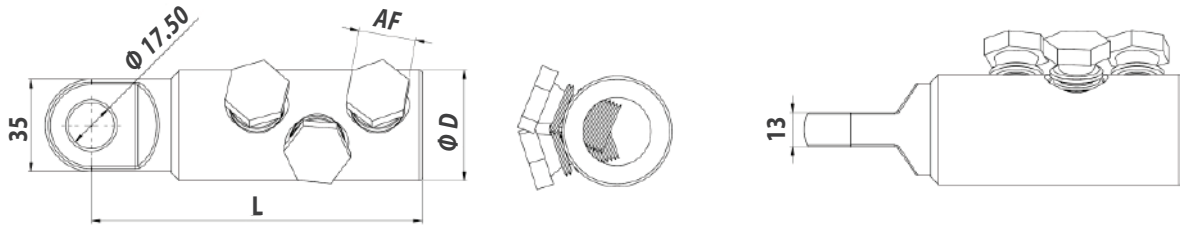
DIMENSION INFORMATION OF "SBC-B SERIES"
