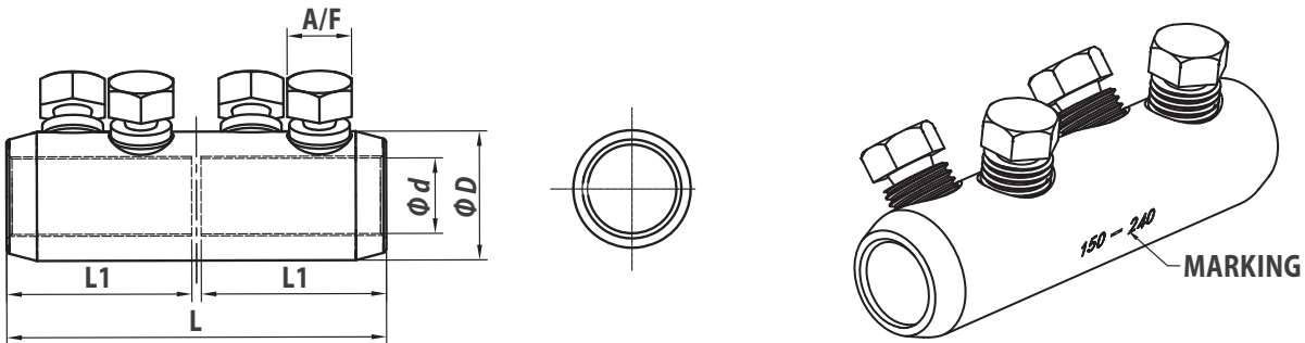
DIMENSION INFORMATION OF "SBSC"
