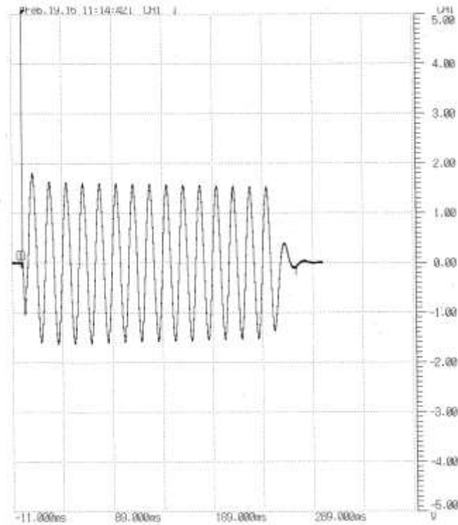
A11&A12 10kA/0.27sec
