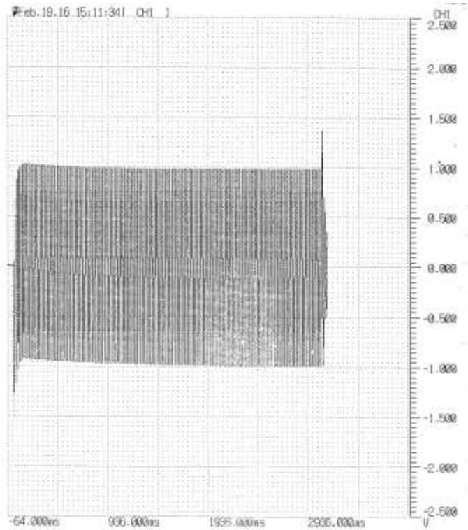
A1&A2 3.5kA/3.05sec
